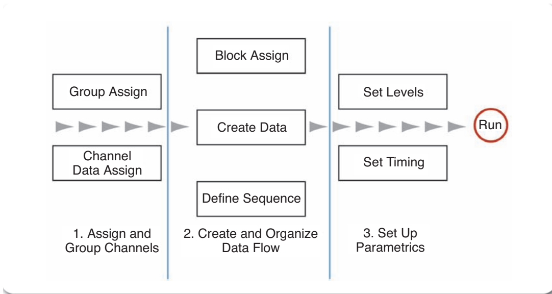
▶ Figure 50. Steps to create digital signals using a logic signal source.
