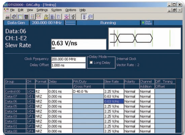
► Figure 49. Editing/control screen.
