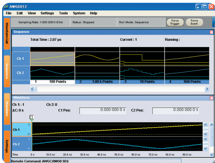
▶ Figure 33. The Graphic editor and Sequence editor are combined for flexible waveform creation.
