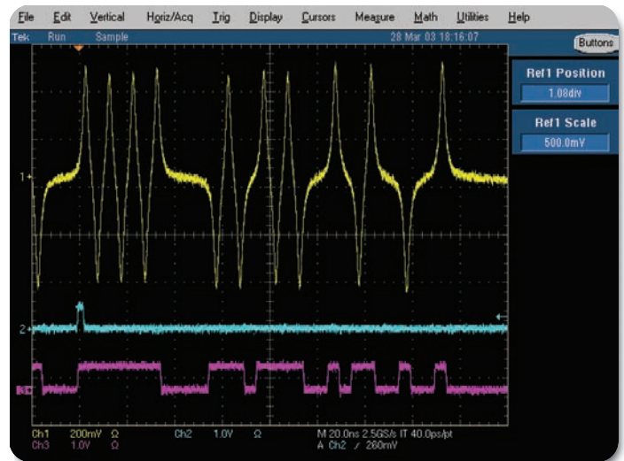
► Figure 29. Marker outputs.
