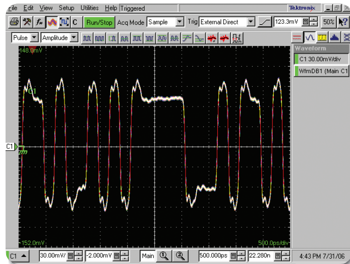
▶ Figure 37. 5 Gbps pre/de-emphasized signal.
