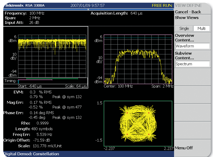
► Figure 40. EVM/Constellation measurement.
