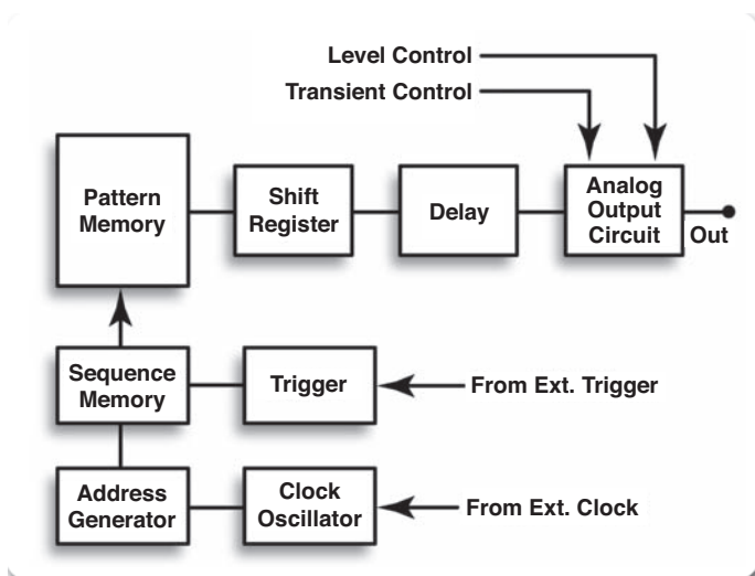
► Figure 41. The architecture of a PPG or DTG (simplified).
