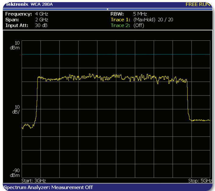
► Figure 39. UWB (MBOA) three band (480 Mbps 1795 MAC bytes 96 symbol payload).
