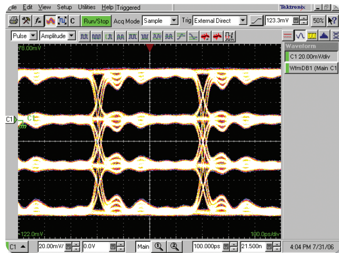
▶ Figure 38. 20 Gbps 4PAM signal.
